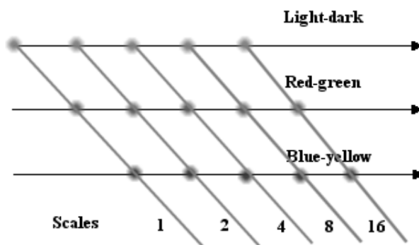
Figure 2. In a dyadic scale space decomposition of a color opponent model-based image, a given scale s_0 will be characterized by feature of the scale s for the light-dark channel, 2 \times s_0 for the red-green channel, 4 \times s_0 for the blue-yellow one.
